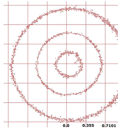
Iso-Illuminance Diagram (Flat Surface Distribution)
