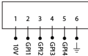
Figure 3.4: GPI Pinout
